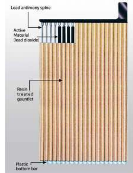
Tubular Plate and its various components
